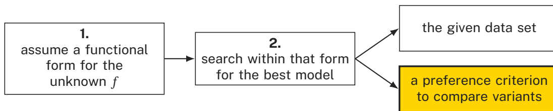
Figure 3. Every algorithm assumes a form for f , then searches within it using the data and a preference criterion.
