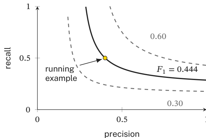
Figure 5. Curves of constant F_1 in the precision and recall plane. The marked point is the running example, F_1 = 0.444 .
