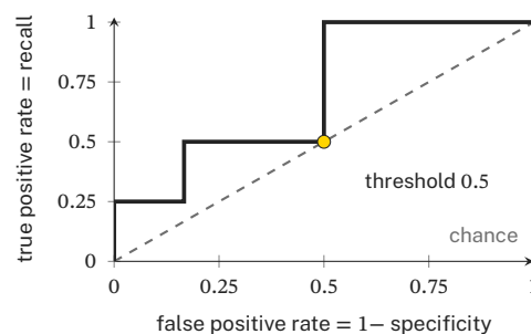
Figure 6. ROC curve for the running example. The marked point is the threshold 0.5, on the chance diagonal. AUC = 17/24 = 0.708 .
